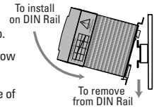
fig.1 Mounting on DIN Rail
